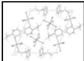
Fig. 2. The crystal structure packing scheme viewed along [100] showing the hydrogen bonds system.
